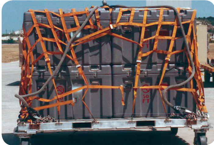
463L INTEX (Internal/External) Multipurpose Aircraft/Helicopter Pallet shown with optional casters and cargo net
