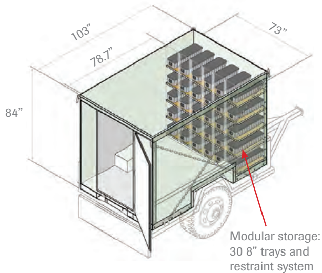
Interior of M105 Trailer Shop Container
