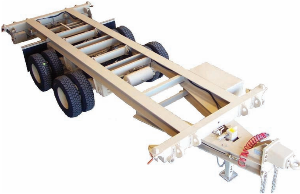
Full length view of the AAR/MCT ISO Mobility Trailer P/N: 1103-4000-00.
