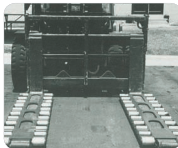
This particular model attaches to a forklift and is used with dunnage at the aircraft for loading. Note the rubber protected nose plate.
