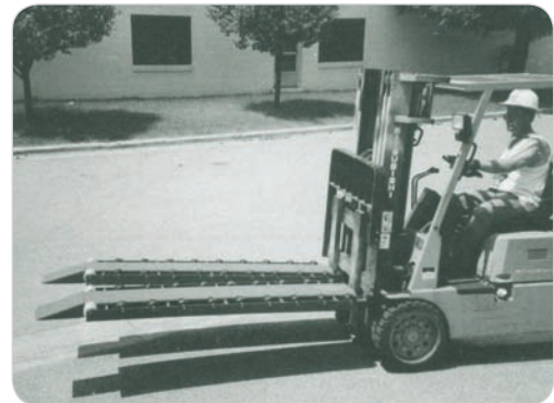
This particular model attaches to a forklift and is used to pick up pallets directly from the ground. Note the beveled nose plate.
