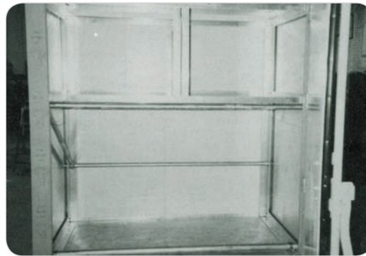
Full-size ISU Tire Rack (P/N 60041-003) shown in ISU Two Door Container.
